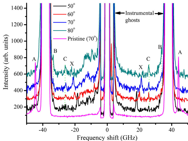
Fig. 5. SBS spectra for the implanted diamond after annealing at 1200^\circ\text{C} , incident angles varied between 50^\circ – 80^\circ while maintaining the same wavevector. Spectra are displaced for clarity. Pristine ( 70^\circ ) is the spectrum obtained from pristine diamond from light incident at 70^\circ .
