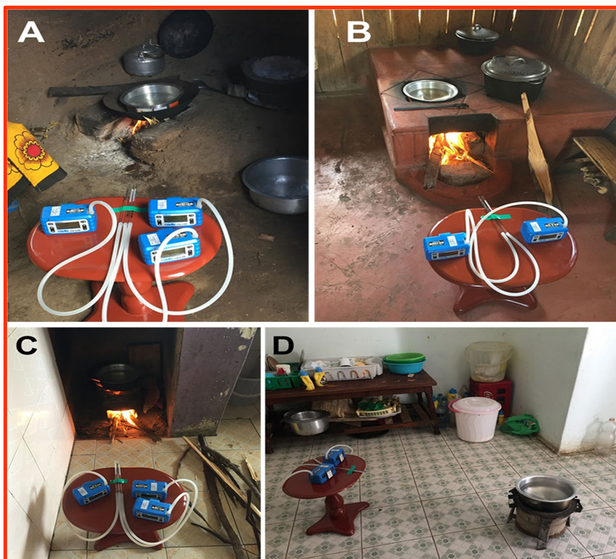
Fig. 3 Typical sampling setup used at A Narok rural HH#1 (improved 3-stone), B Bomet rural HH#1 (improved 3-stone), C Bomet urban HH#1 (Jiko), and D Narok urban HH#2 (Jiko). For all samples, the PDMS trap was positioned at 65 cm from the stove and at a height of 36 cm above the ground
