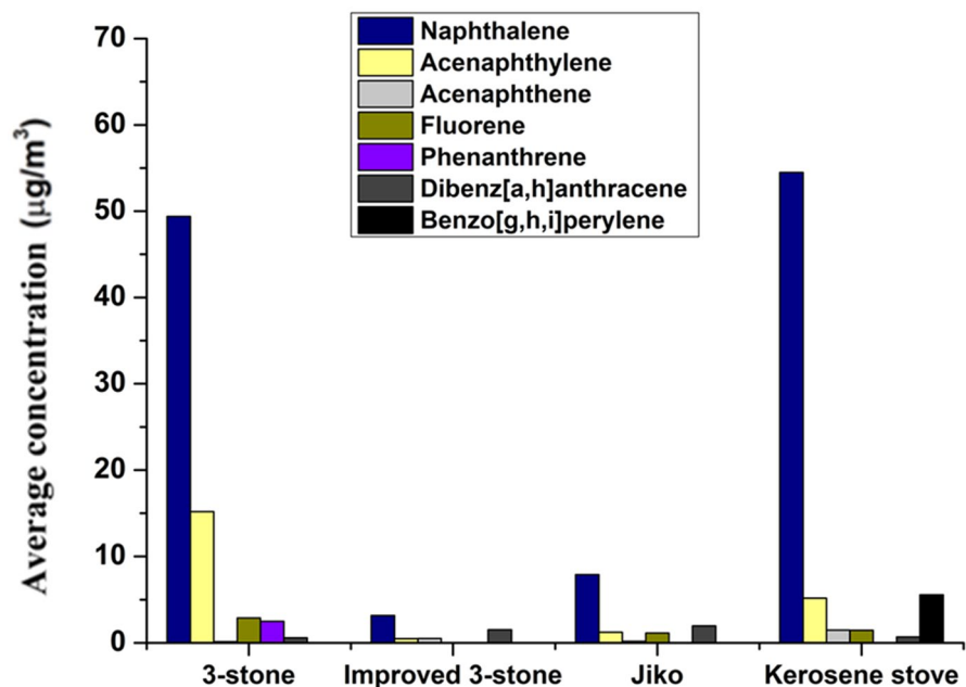
Fig. 5 Average gaseous PAH concentrations from various combustion devices. N_{(3\text{-stone})} = 3 , N_{(\text{Improved } 3\text{-stone})} = 3 , N_{(\text{Jiko})} = 8 , N_{(\text{Kerosene stove})} = 2 . LOQs were used in the average calculation where [\text{analyte}] < \text{LOQ}
