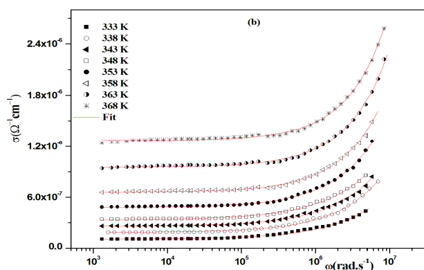
Figure 4. AC Electrical Behaviour of Conducting Solids and Liquids as Dimensional Frequency Exponent Parameter
